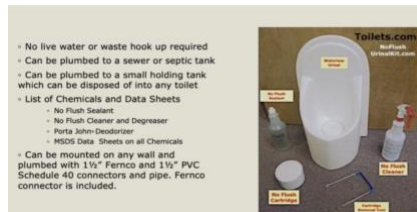
No Flush Urinal Kit Installed Ships with Supplies For 10,000 Uses
